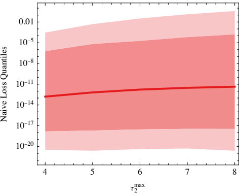
N=1 Minimal Model: m=5, \Delta_{\max}=4
