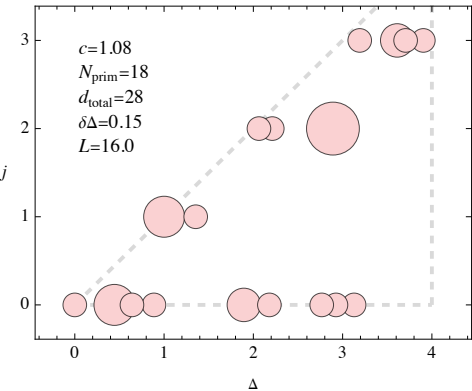
Spectrum After Optimization: c=1.08 , \Delta_{\text{gap}}=0.44
