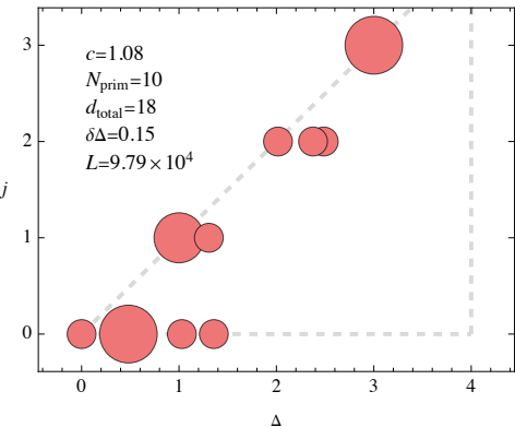
Spectrum After Optimization: c=1.08 , \Delta_{\text{gap}}=0.48
