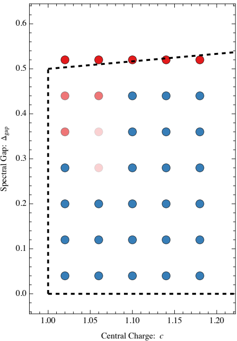
\Delta_{\max}=5 Spectra Truncated to \Delta_{\max}=4
