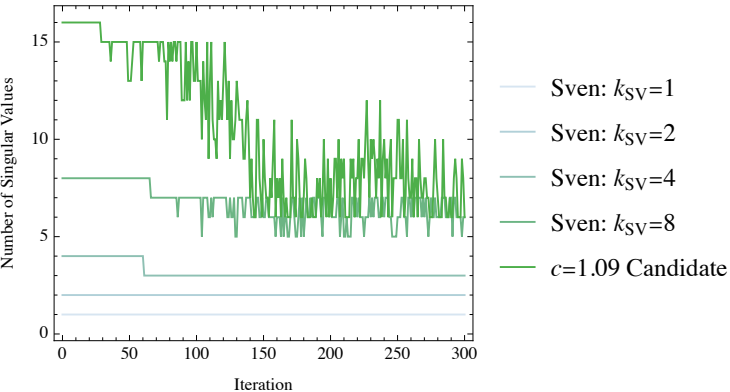
Sven: Adaptive Singular Value Selection
