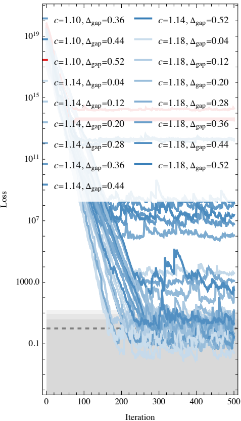
Test Loss Evolution: Singular Value Descent
