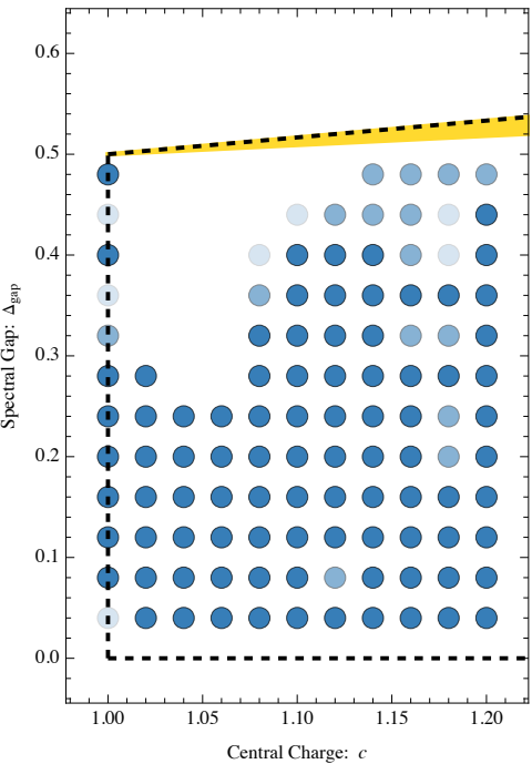
Survey Results: Candidate 2D CFTs, \Delta_{\max}=4
