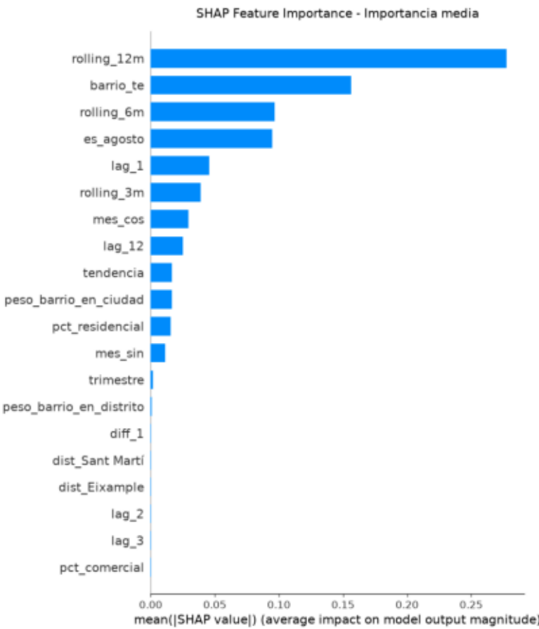
SHAP: importancia de features
