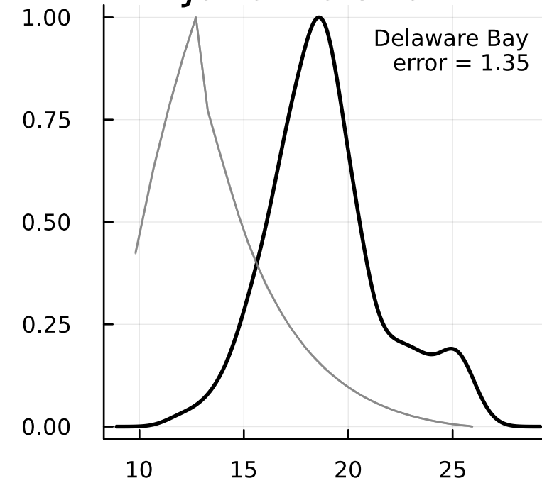
Juvenile-site fit
