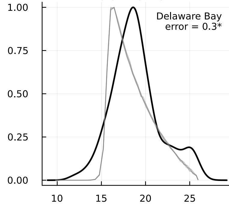
Adult-site fit
