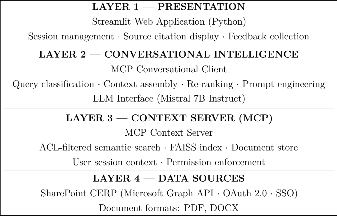
Figure 4.1: AntiGravity four-layer architecture overview
