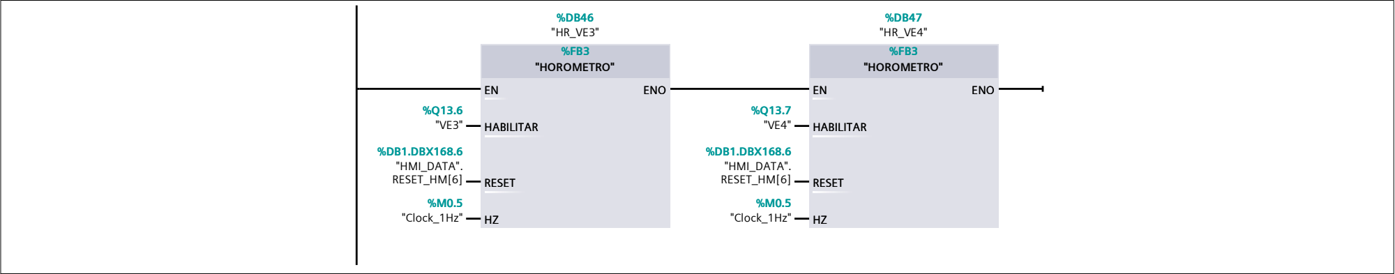
Network 28:
