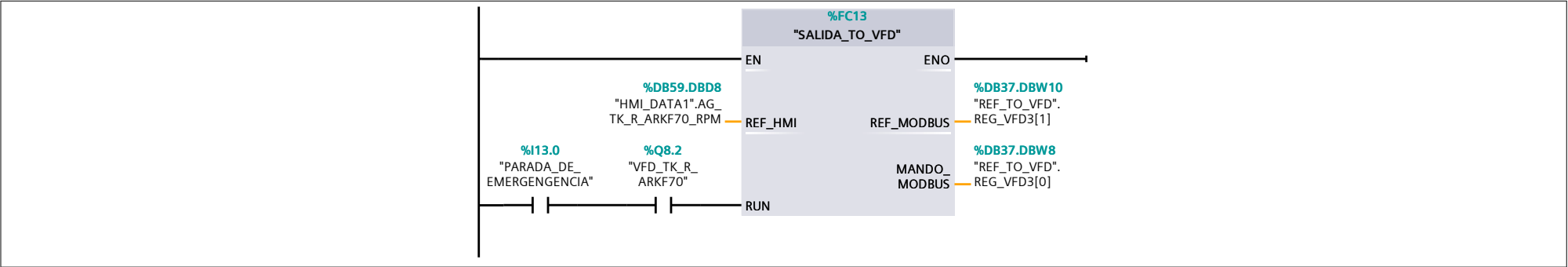
Network 25:
