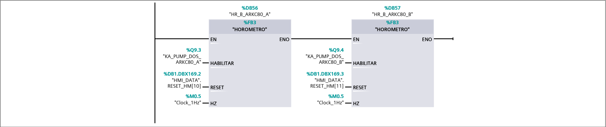
Network 33:
