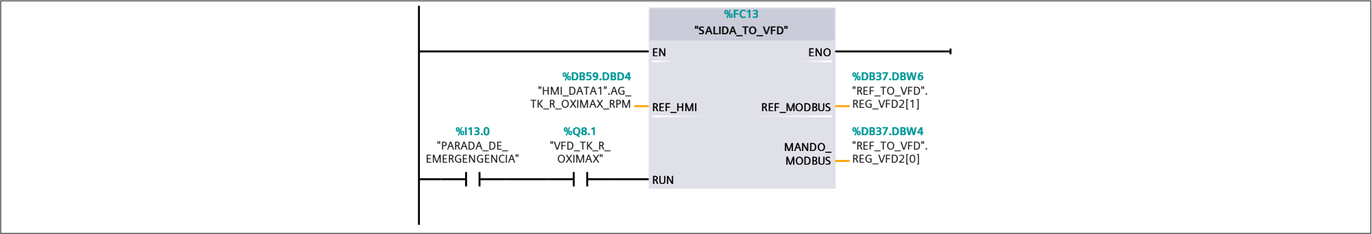
Network 24:
