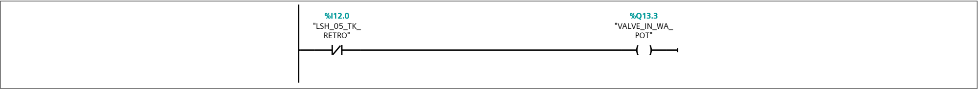
Network 34:
