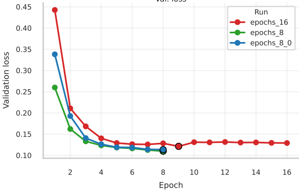
Val. loss
