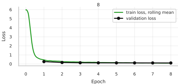
Train vs validation loss
