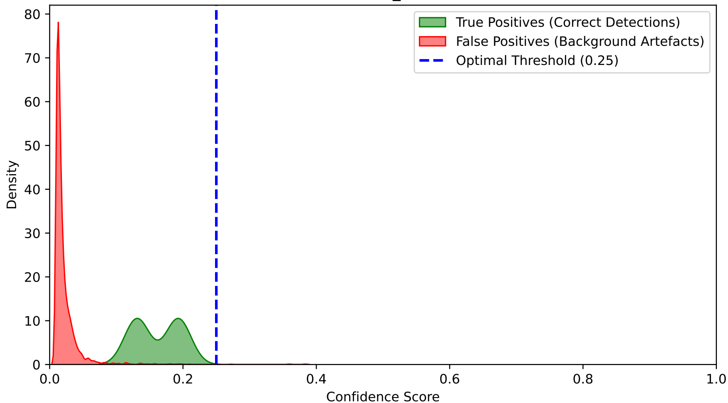
Overlapping Confidence Score Distribution (RTDETR clahe scratch Cycle 4) Class: Small_Mammal
