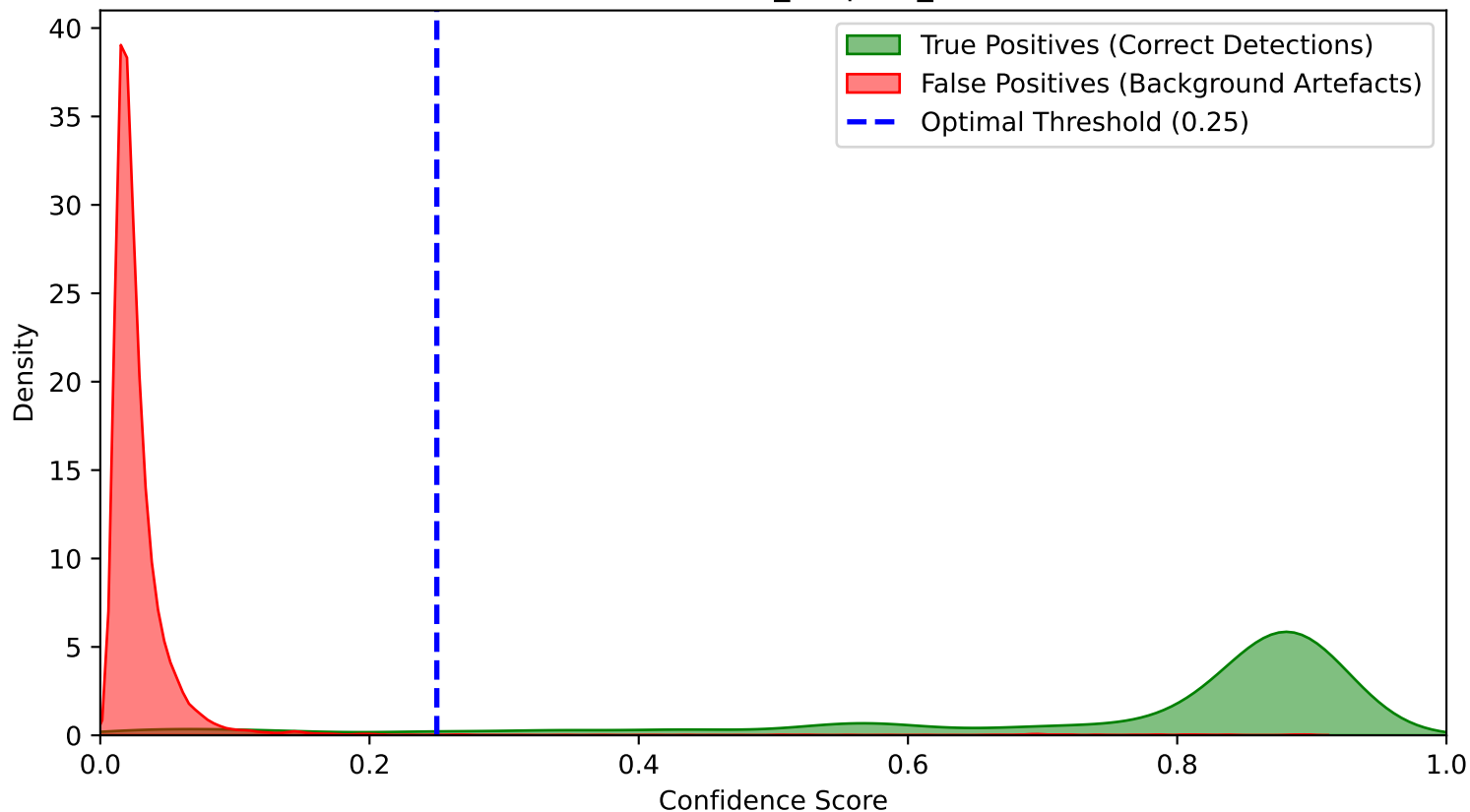
Overlapping Confidence Score Distribution (RTDETR plain scratch Cycle 4) Class: Western_Leopard_Toad
