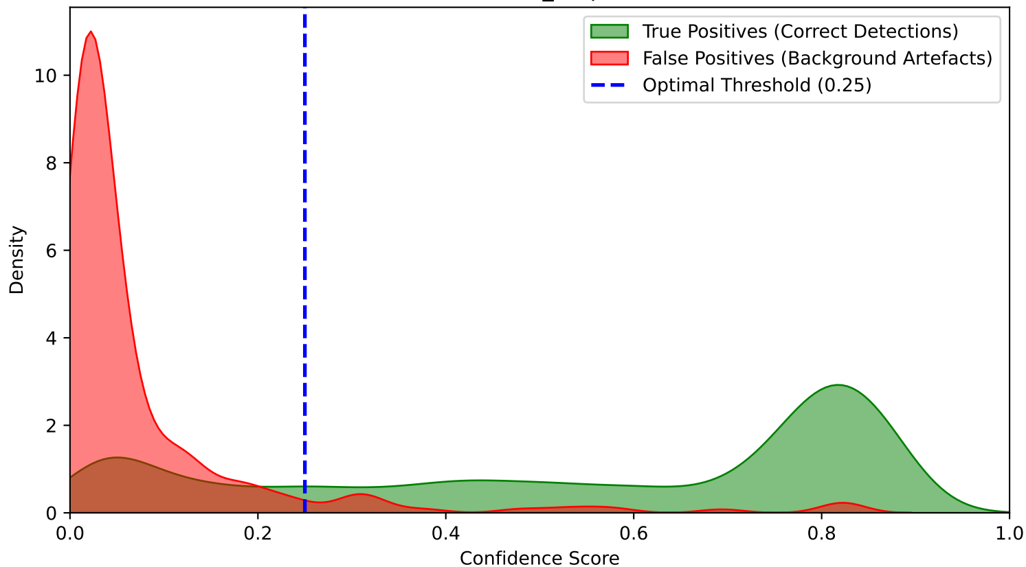
Overlapping Confidence Score Distribution (YOLO clahe scratch Cycle 4) Class: Other_Amphibian
