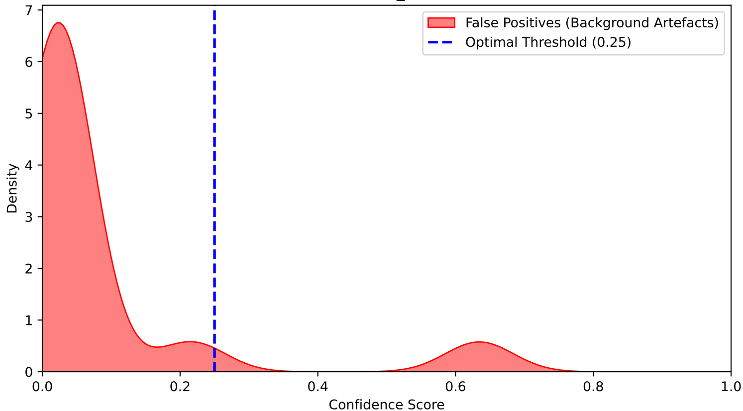
Overlapping Confidence Score Distribution (YOLO clahe scratch Cycle 4) Class: Small_Mammal
