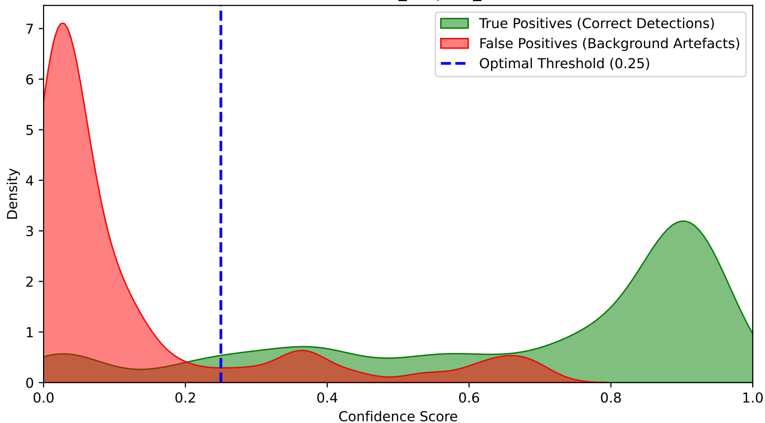
Overlapping Confidence Score Distribution (YOLO clahe scratch Cycle 4) Class: Western_Leopard_Toad
