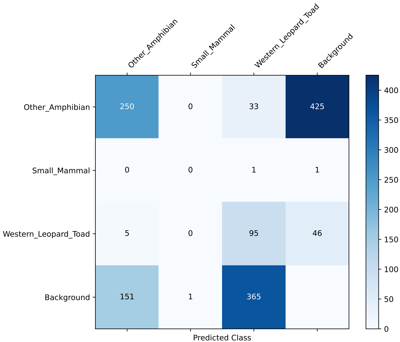
Confusion Matrix: FASTER_RCNN (Optimal Thresholds)
