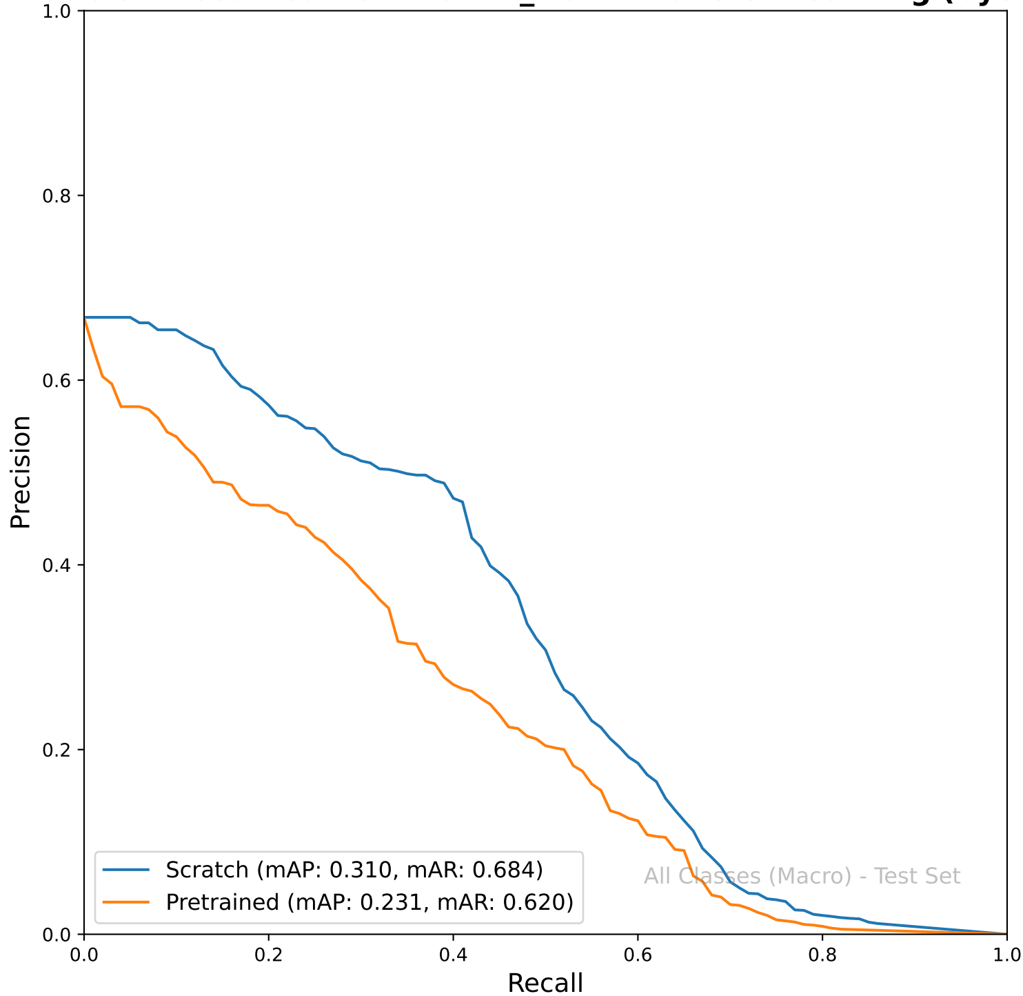
Precision-Recall Curve: FASTER_RCNN Transfer Learning (Cycle
