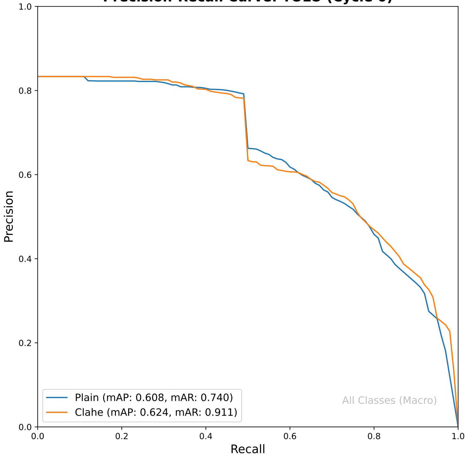
Precision-Recall Curve: YOLO (Cycle 0)
