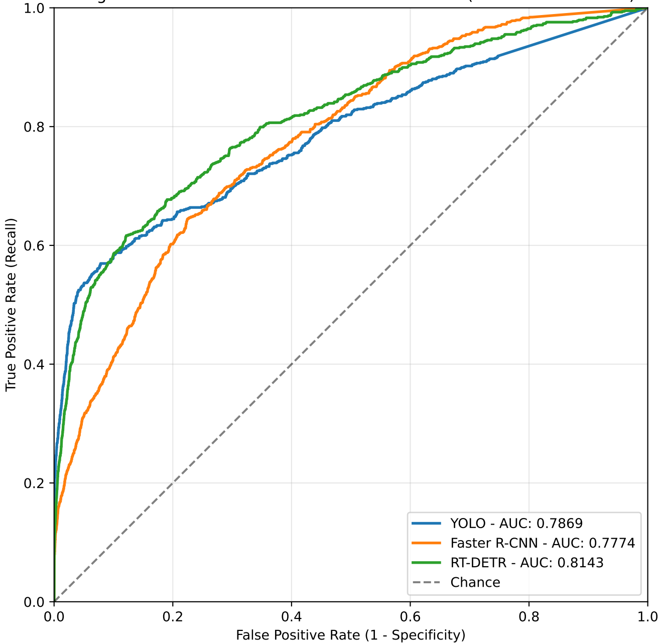
Image-Level ROC Curves - Baseline Architectures (Test Unlabeled Pool)
