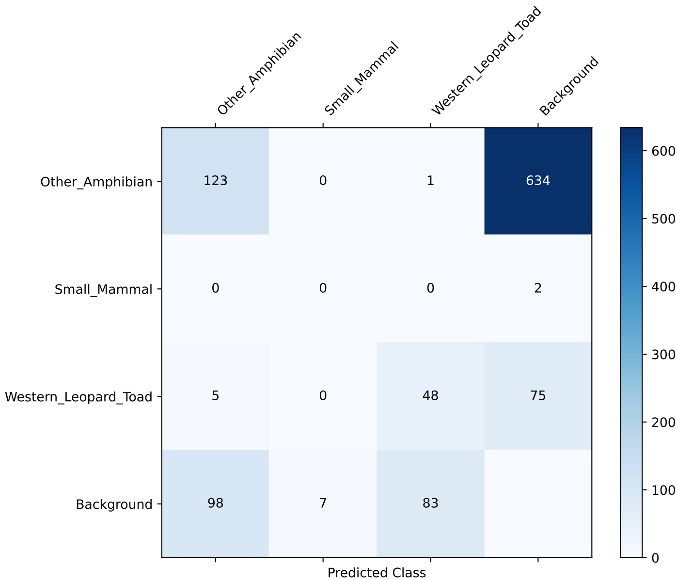
Confusion Matrix: YOLO (Threshold=0.5)
