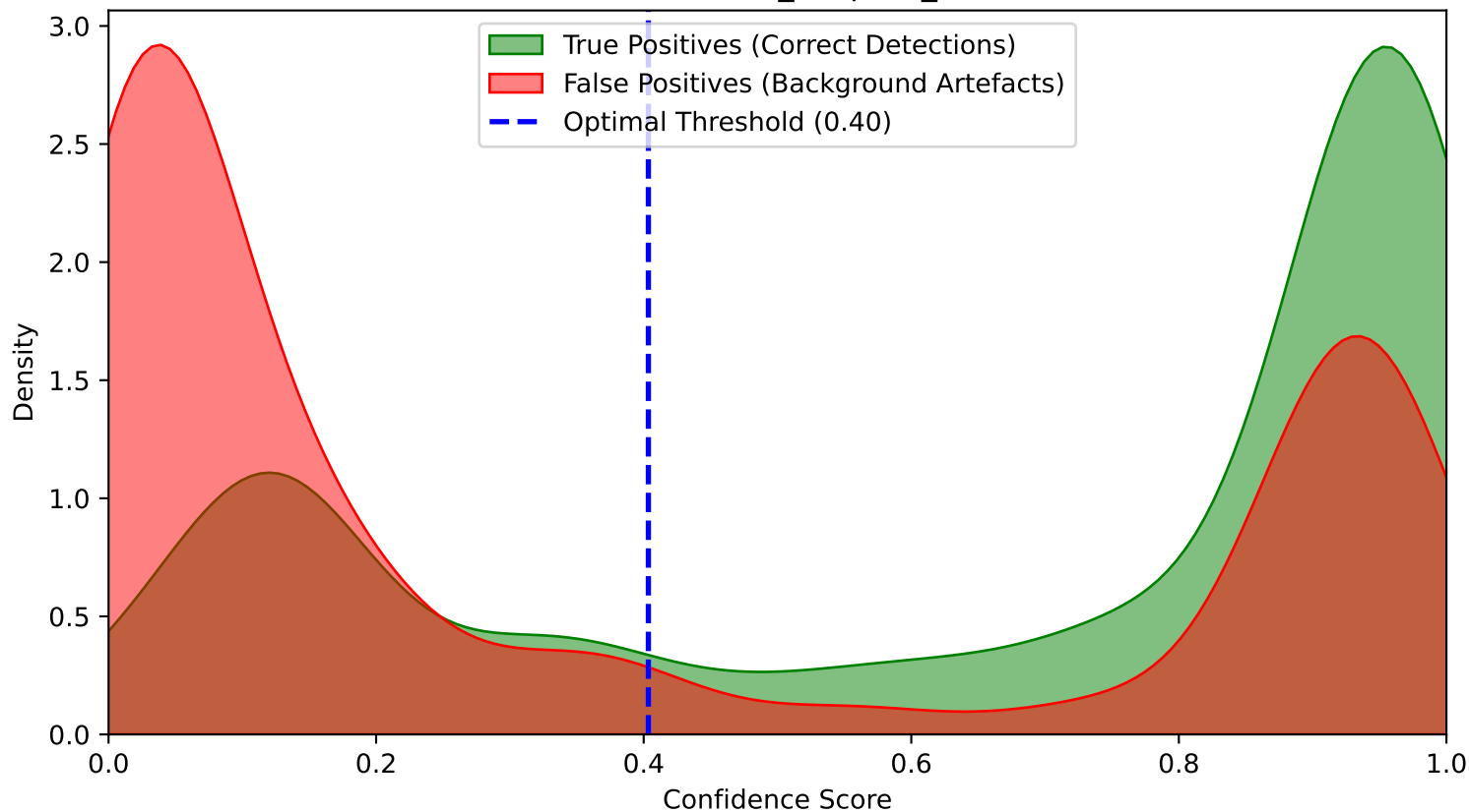
Overlapping Confidence Score Distribution (YOLO clahe pretrained Cycle 4) Class: Western_Leopard_Toad
