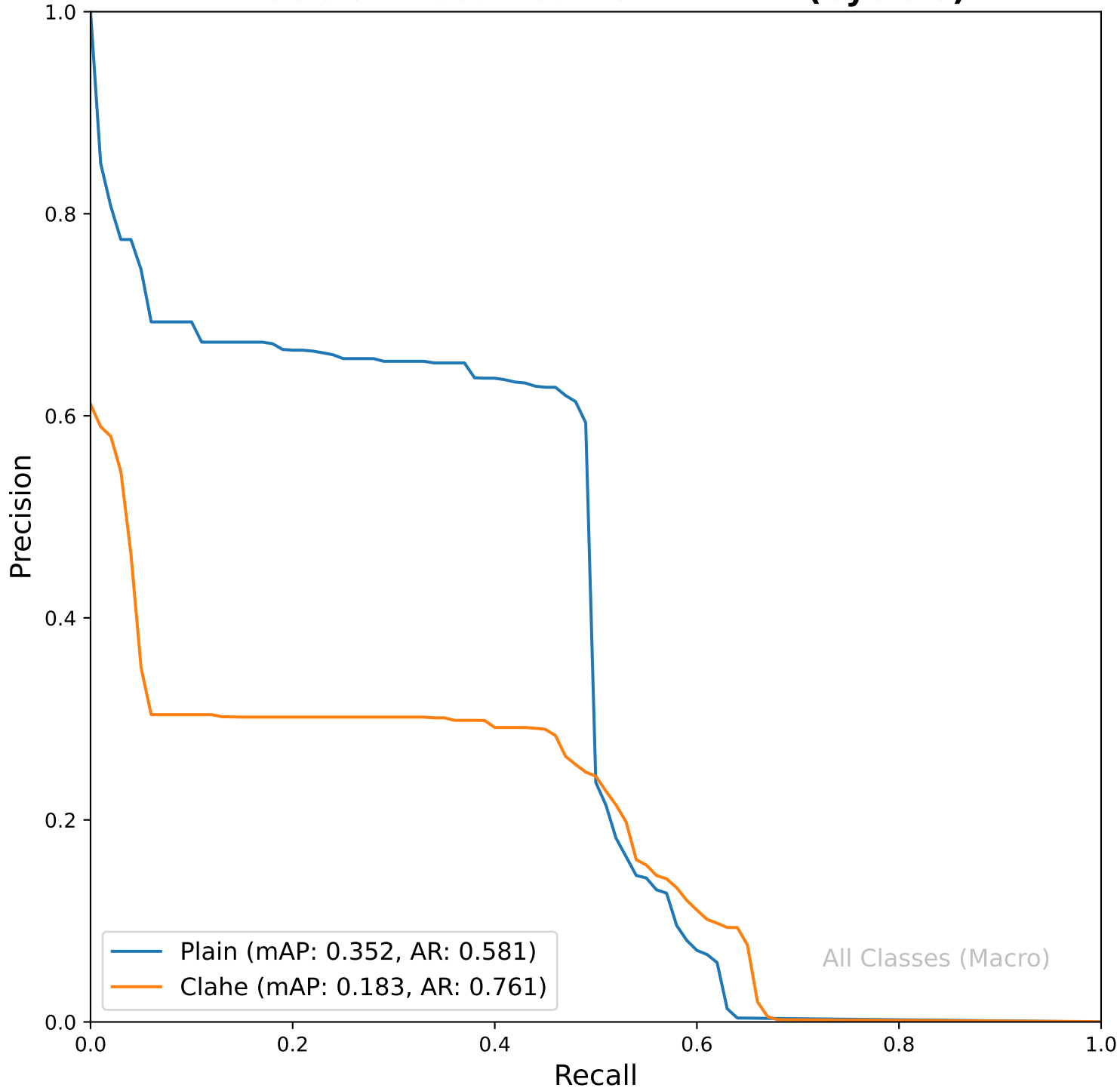
Precision-Recall Curve: RTDETR (Cycle 0)
