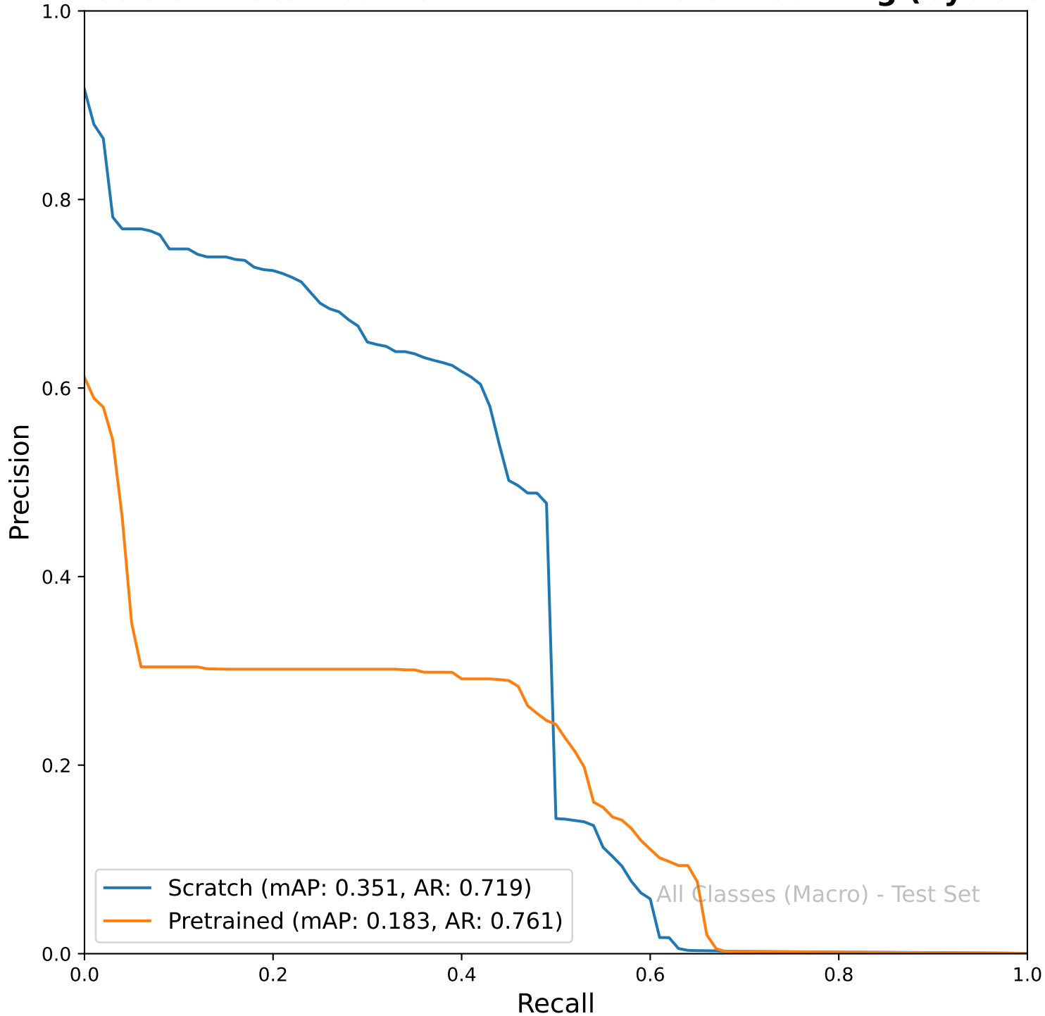
Precision-Recall Curve: RTDETR Transfer Learning (Cycle 0)
