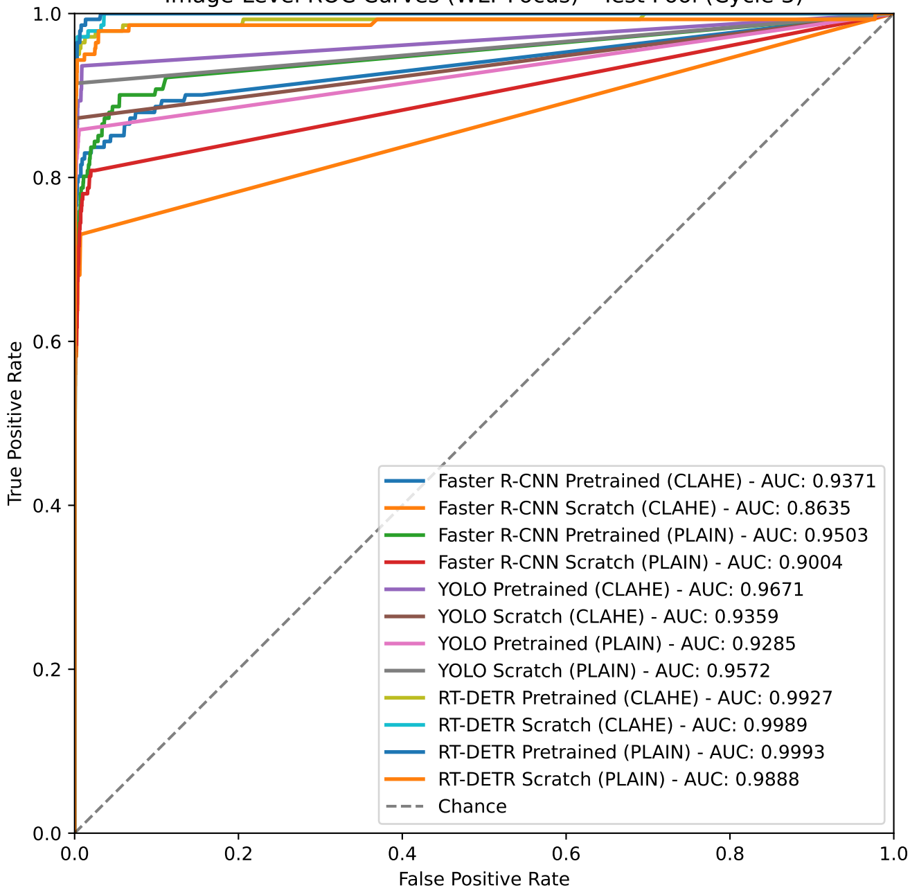
Image-Level ROC Curves (WLT Focus) - Test Pool (Cycle 3)
