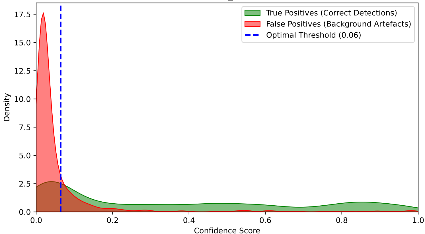
Overlapping Confidence Score Distribution (FASTER_RCNN clahe pretrained Cycle 4) Class: Other_Amphibian
