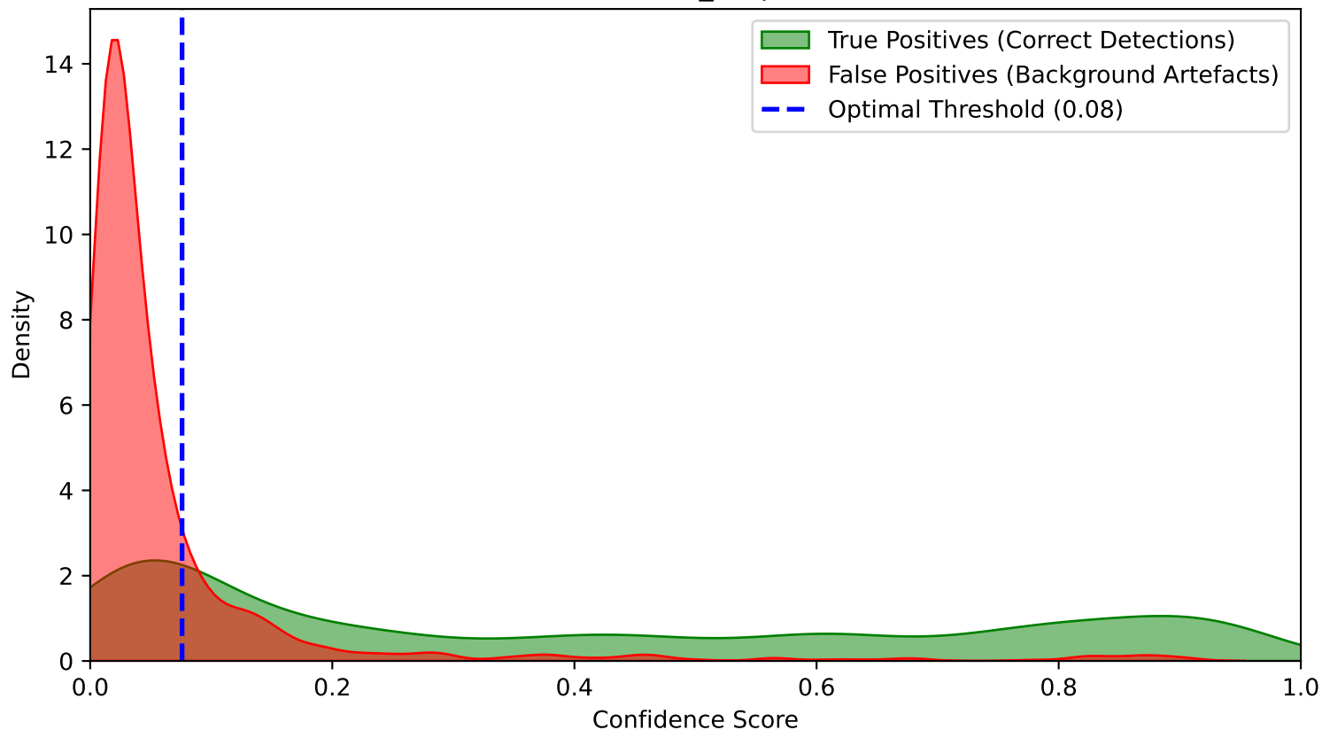
Overlapping Confidence Score Distribution (FASTER_RCNN clahe scratch Cycle 4) Class: Other_Amphibian
