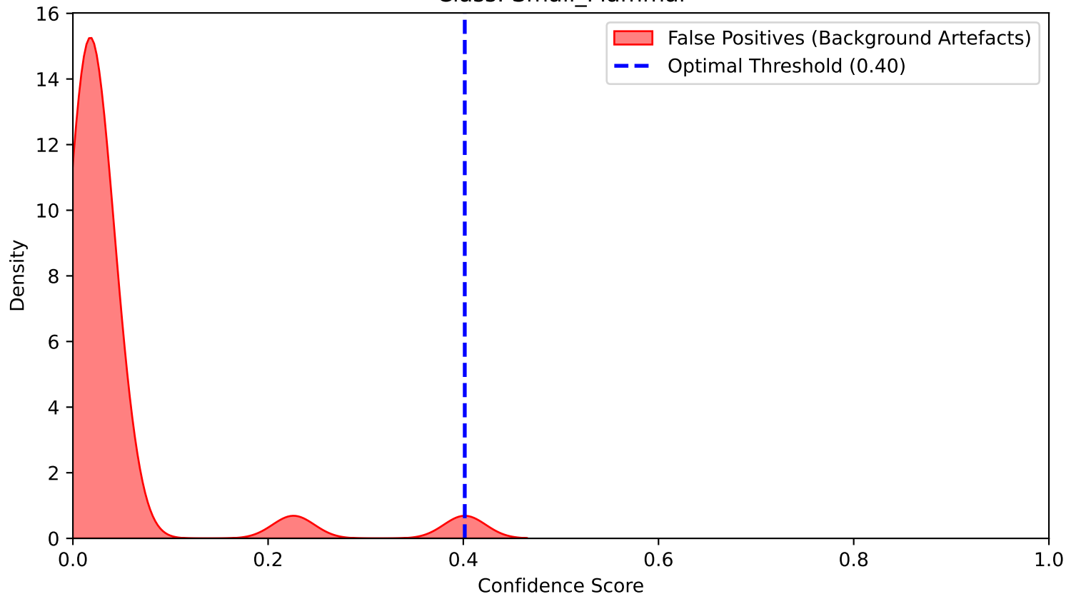
Overlapping Confidence Score Distribution (FASTER_RCNN plain pretrained Cycle 4) Class: Small_Mammal
