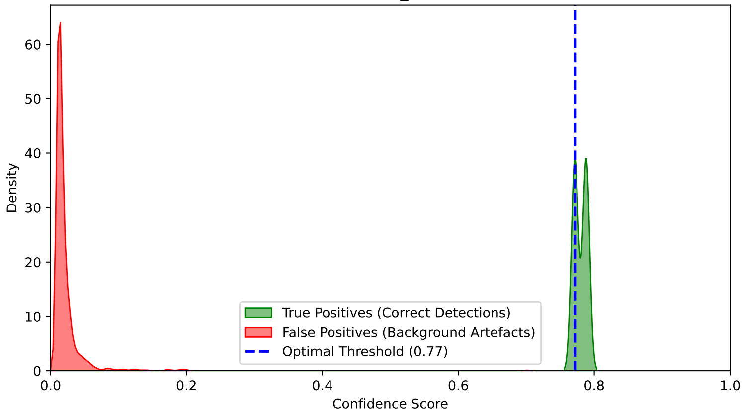
Overlapping Confidence Score Distribution (RTDETR plain pretrained Cycle 4) Class: Small_Mammal
