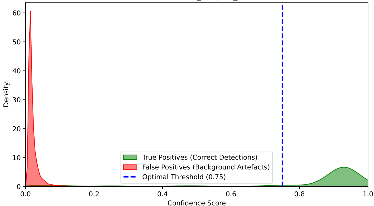
Overlapping Confidence Score Distribution (RTDETR plain pretrained Cycle 4) Class: Western_Leopard_Toad
