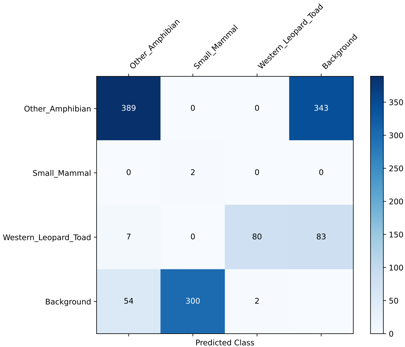
Confusion Matrix: YOLO (Optimal Thresholds)
