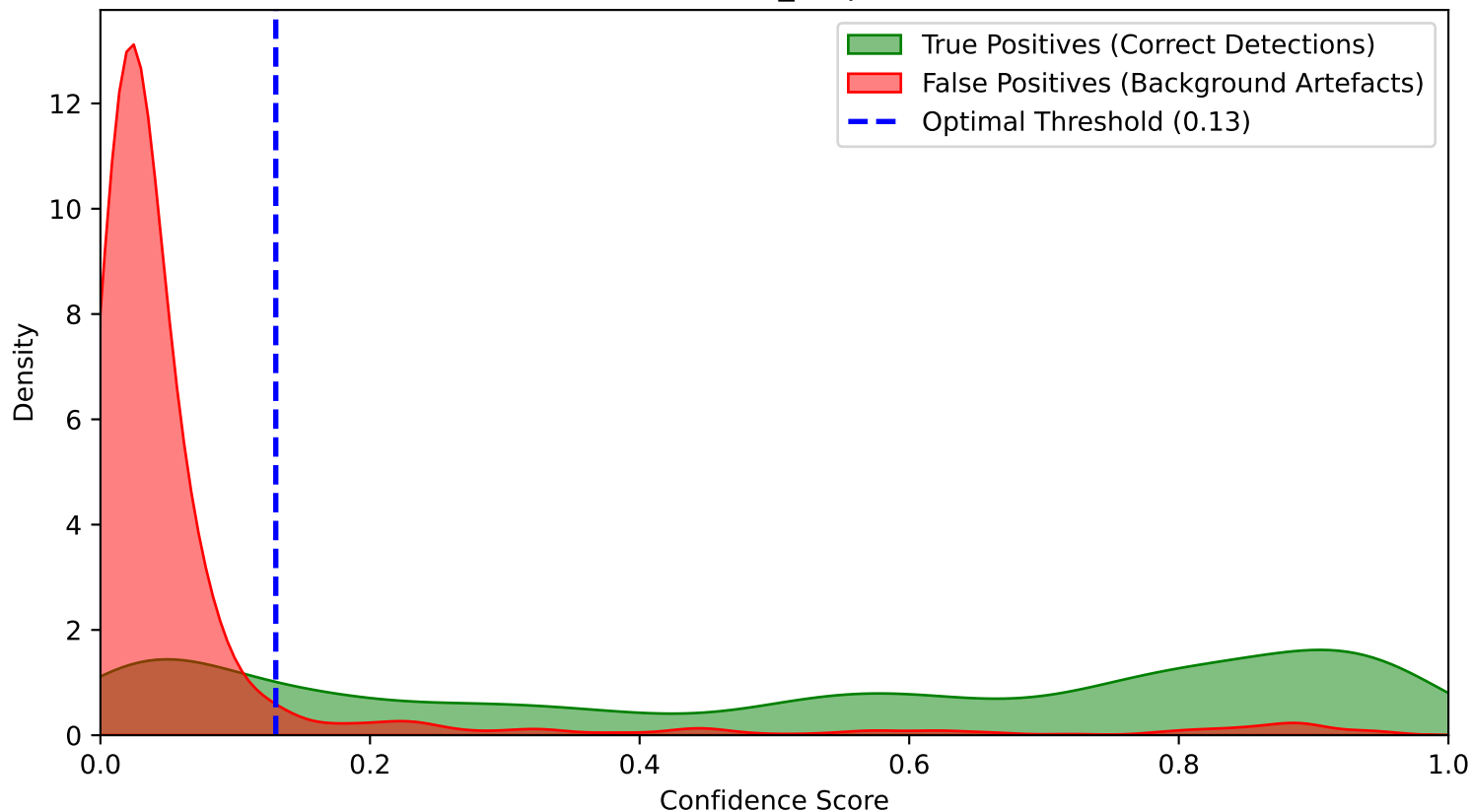
Overlapping Confidence Score Distribution (FASTER_RCNN plain scratch Cycle 4) Class: Other_Amphibian
