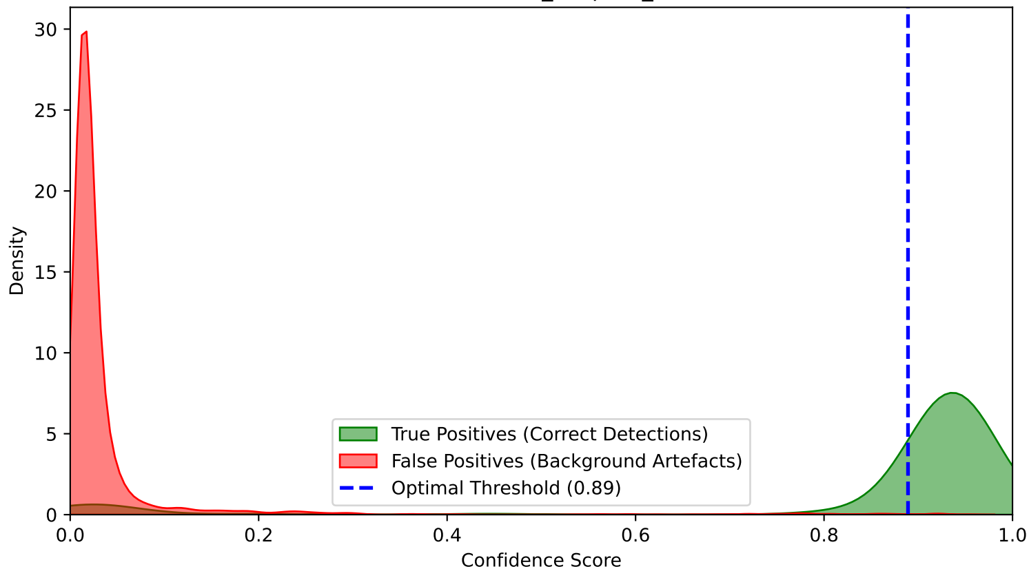
Overlapping Confidence Score Distribution (RTDETR clahe pretrained Cycle 4) Class: Western_Leopard_Toad
