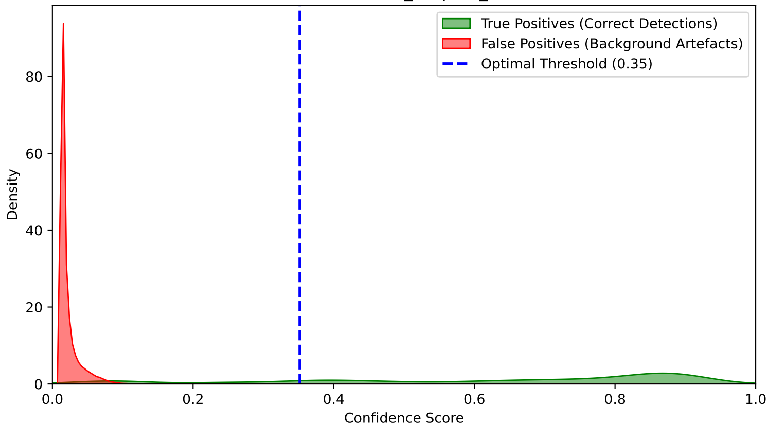
Overlapping Confidence Score Distribution (RTDETR clahe scratch Cycle 4) Class: Western_Leopard_Toad
