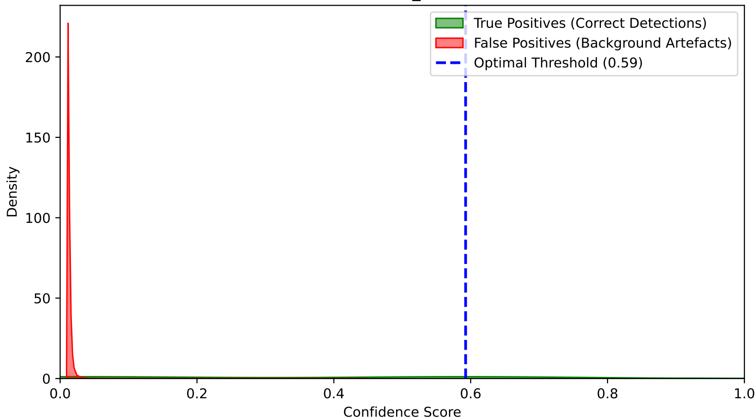
Overlapping Confidence Score Distribution (RTDETR plain scratch Cycle 4) Class: Small_Mammal
