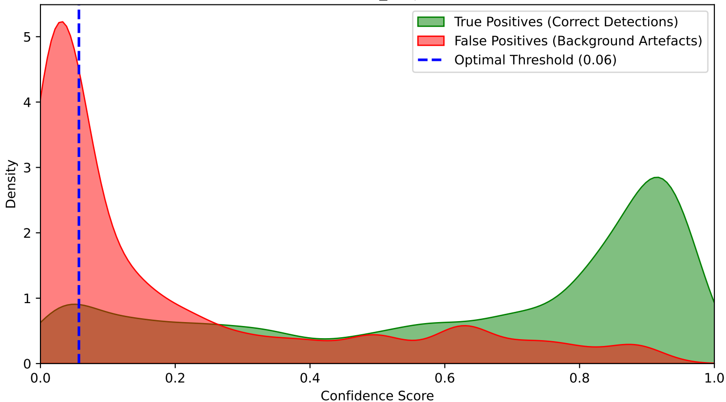
Overlapping Confidence Score Distribution (YOLO clahe pretrained Cycle 4) Class: Other_Amphibian
