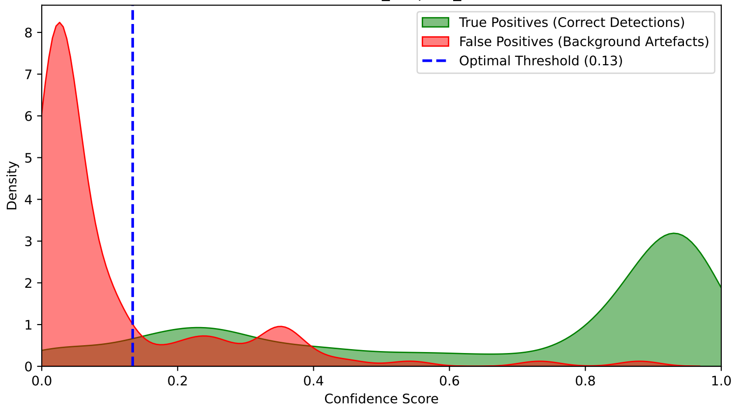
Overlapping Confidence Score Distribution (YOLO plain pretrained Cycle 4) Class: Western_Leopard_Toad
