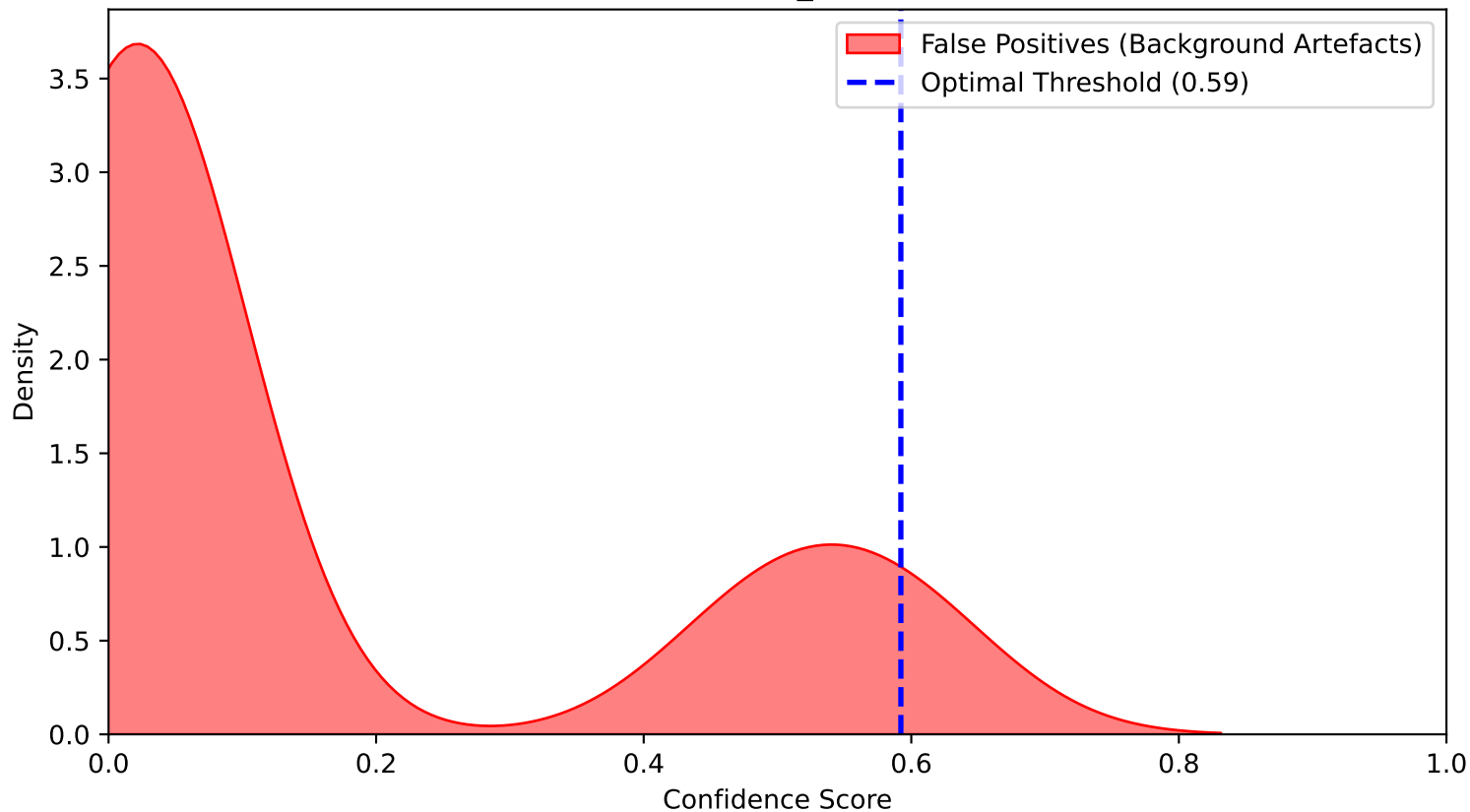
Overlapping Confidence Score Distribution (YOLO plain scratch Cycle 4) Class: Small_Mammal
