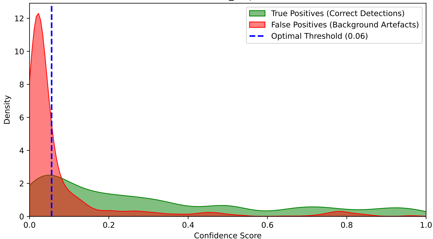
Overlapping Confidence Score Distribution (FASTER_RCNN plain pretrained Cycle 4) Class: Other_Amphibian
