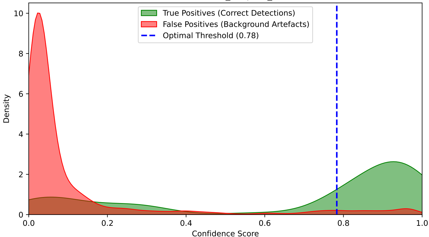
Overlapping Confidence Score Distribution (FASTER_RCNN plain scratch Cycle 4) Class: Western_Leopard_Toad
