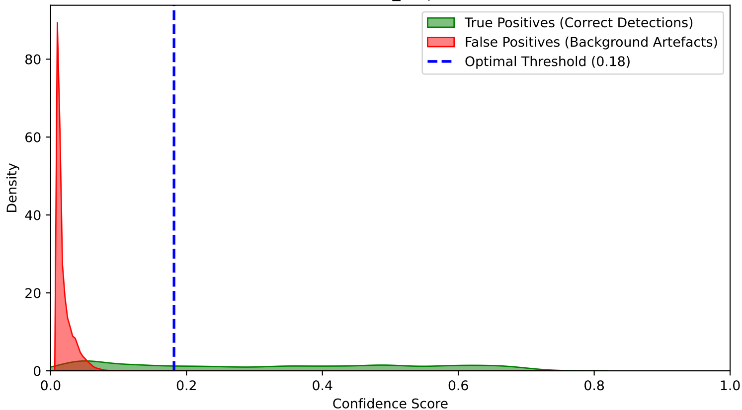
Overlapping Confidence Score Distribution (RTDETR plain scratch Cycle 4) Class: Other_Amphibian
