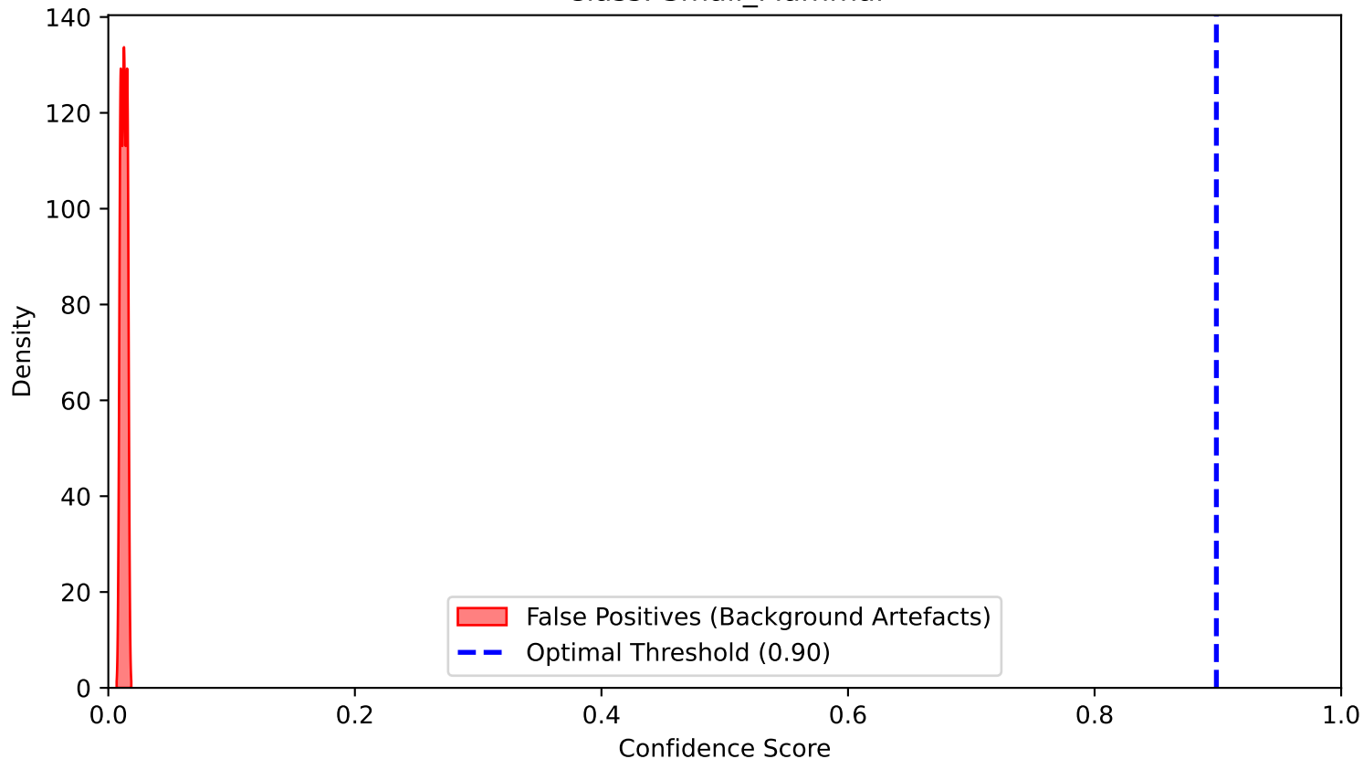
Overlapping Confidence Score Distribution (YOLO clahe pretrained Cycle 4) Class: Small_Mammal
