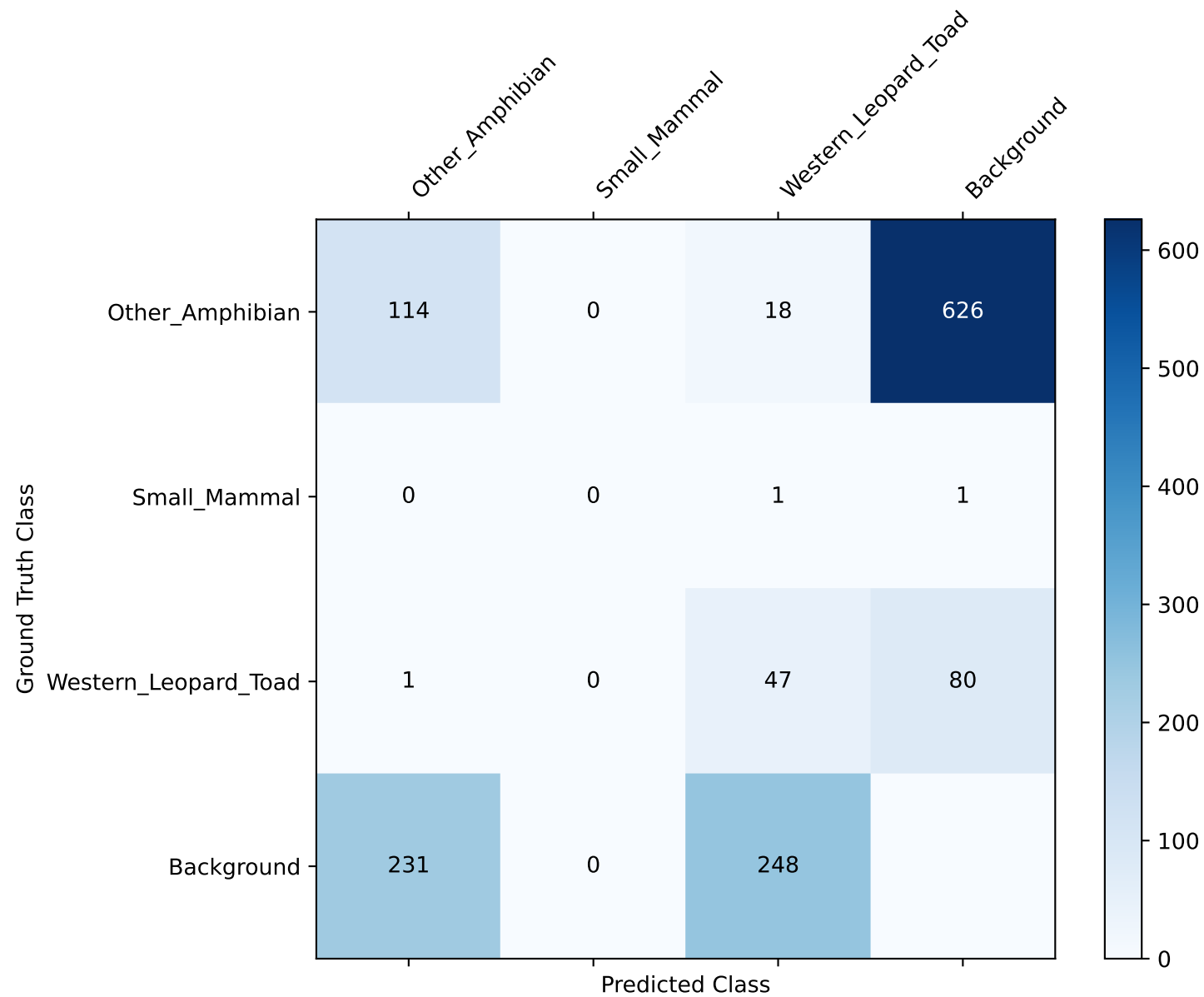
Confusion Matrix: FASTER_RCNN (Threshold=0.5)
