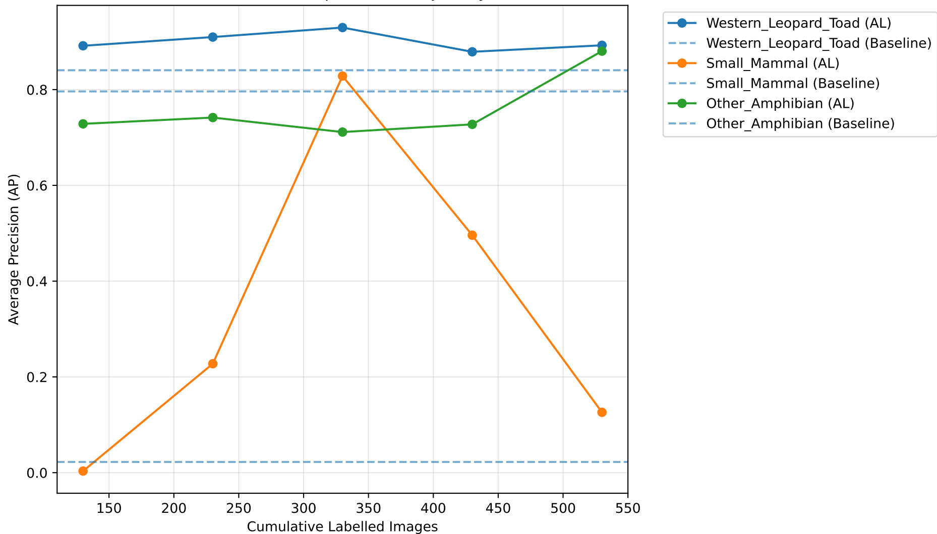
RTDETR Class-Specific AP Trajectory
