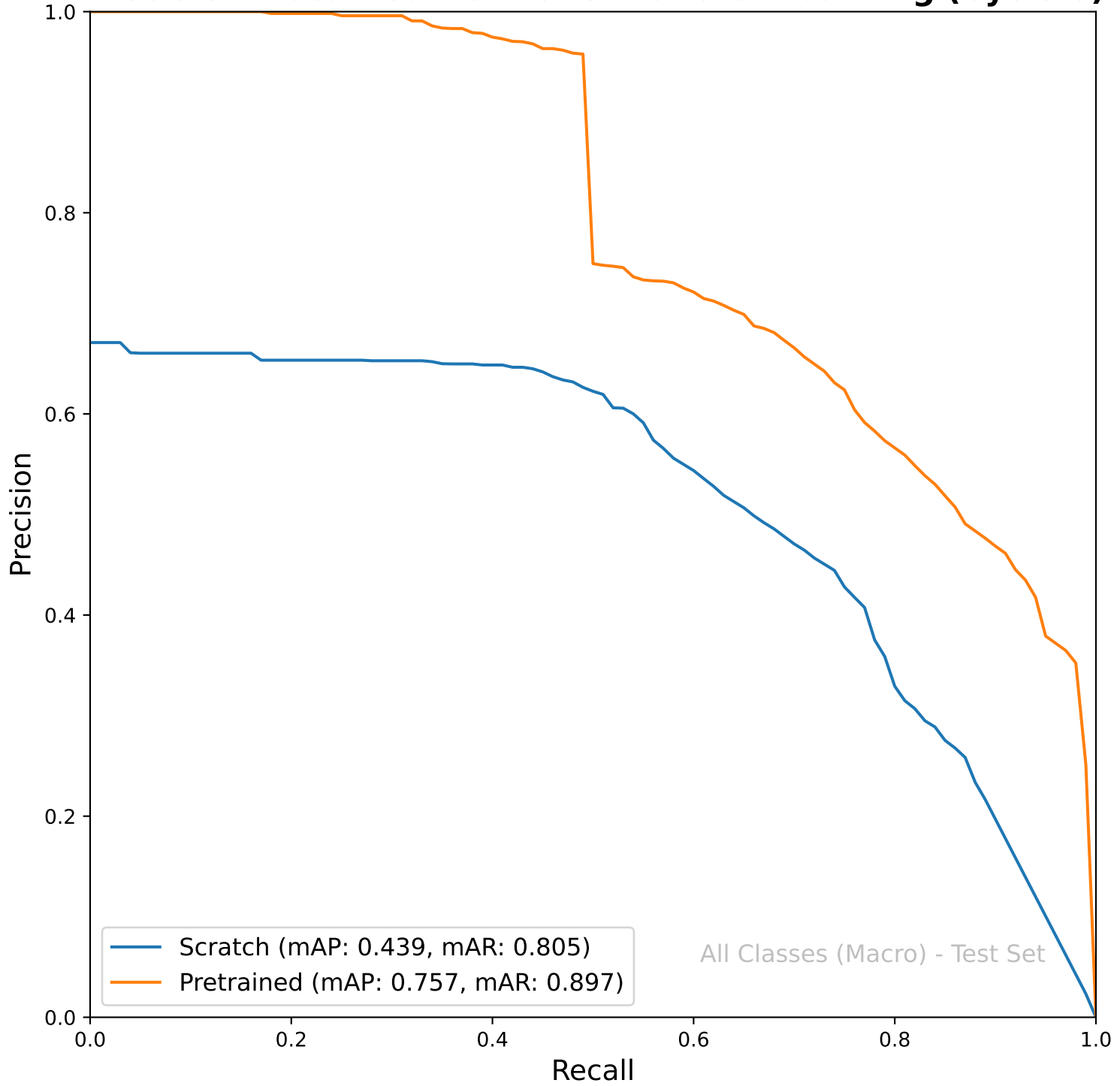
Precision-Recall Curve: YOLO Transfer Learning (Cycle 0)
