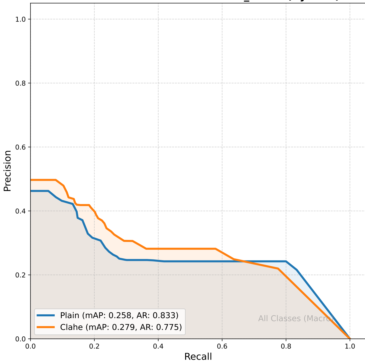
Precision-Recall Curve: FASTER_RCNN (Cycle 0)
