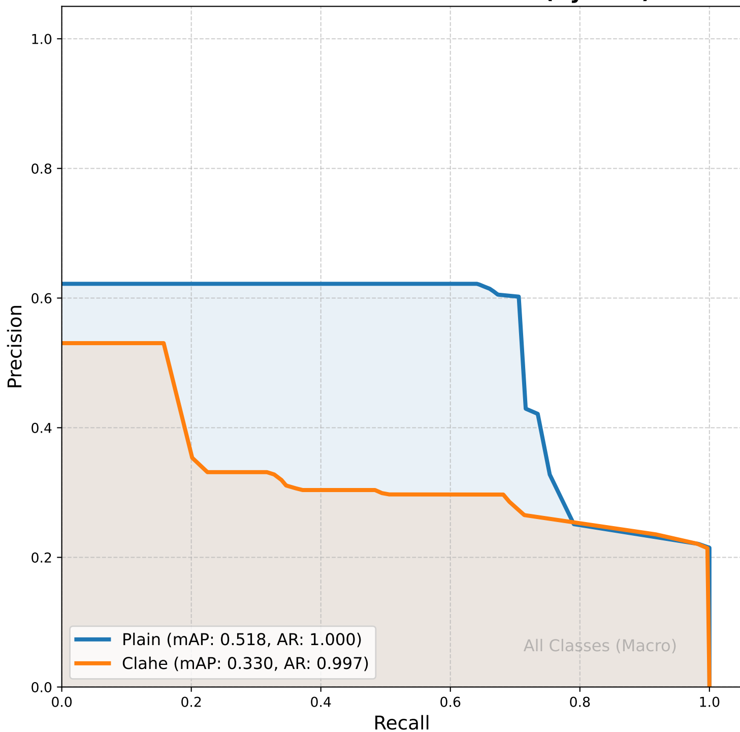
Precision-Recall Curve: RTDETR (Cycle 0)
