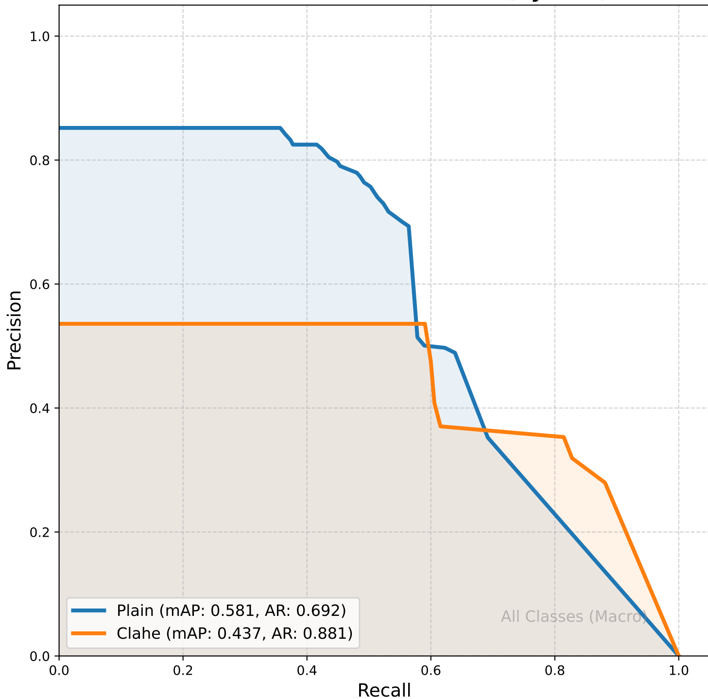
Precision-Recall Curve: YOLO (Cycle 0)
